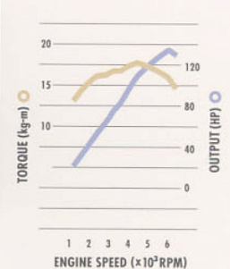
DUAL VVT-i 1.8-liter/Gasoline/Unleaded/2ZR-FE 134HP/6000rpm (SAE net) 17.8kg-m/4400rpm (SAE net)
