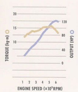
DUAL VVT-i 1.6-liter/Gasoline/Unleaded/1ZR-FE 121HP/6000rpm (SAE net) 15.7kg-m/5200rpm (SAE net)
